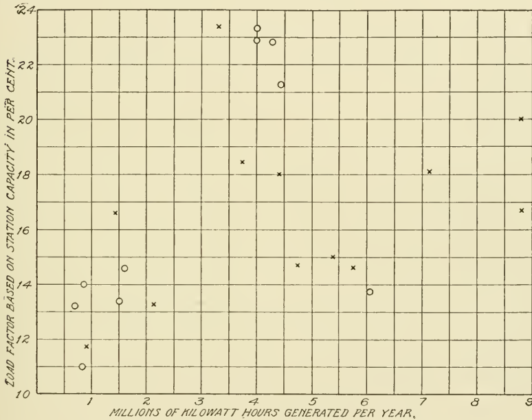
Fig. 166. Load Factor Percentages for Plants of Various Outputs
